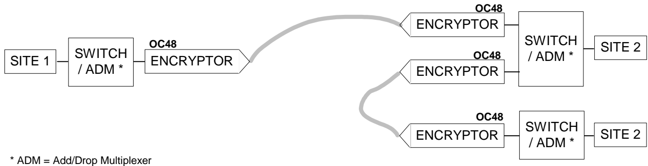
Figure 3. Encryptor Usage Example in Line Encryption Mode.
