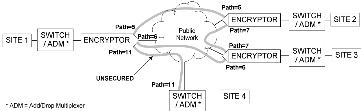
Figure 2. Encryptor Usage Example in Path Encryption Mode.
