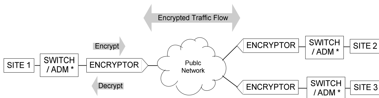
Figure 1. Encrytor Operation.
