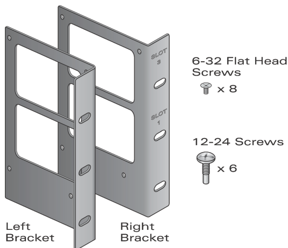
Figure 3-1 Aruba 5000/6000 Rack Mounting Kit
