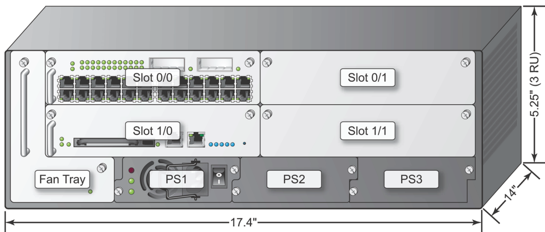
Figure 1-1 The Aruba 5000/6000 Mobility Controller Chassis
