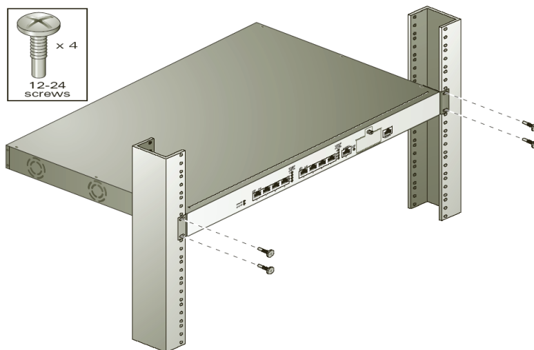
Figure 3-6 Mounting the Aruba 800-series Mobility Controller
