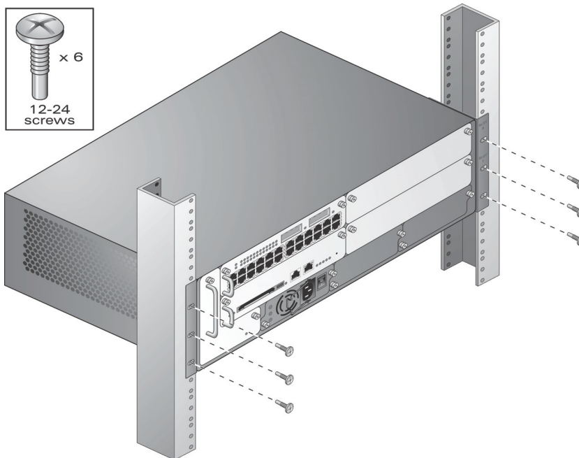
Figure 3-5 Mounting the Aruba 5000/6000 Mobility Controller
