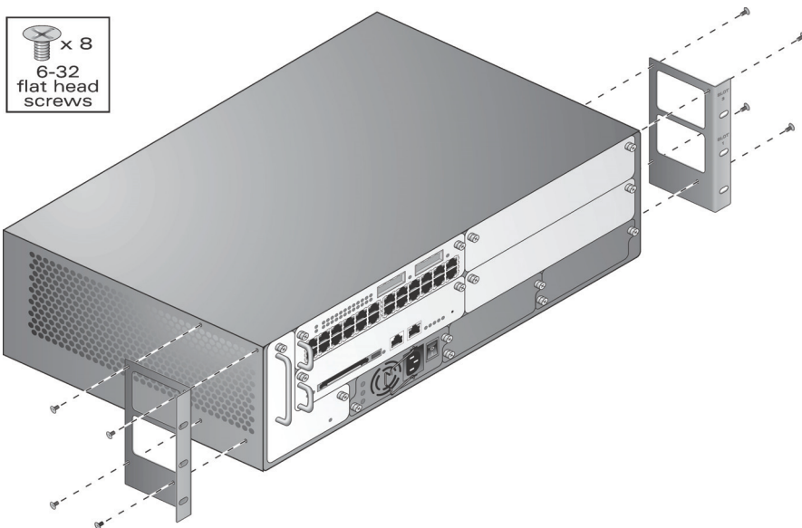
Figure 3-3 Attaching the Rack Mounting Brackets to Aruba 6000
