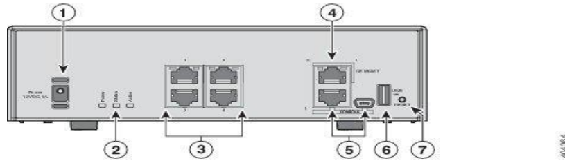
Figure 3 ASA 5506H-X Appliance Rear Panel
