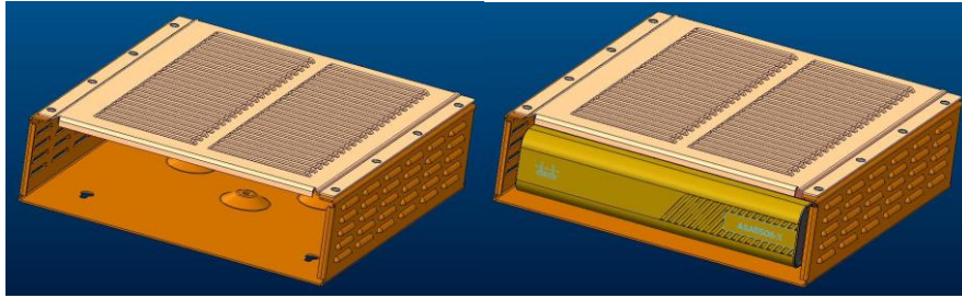
Figure 16 ASA 5506-X, ASA 5506H-X and ASA 5506W-X Opacity Shield Placement
