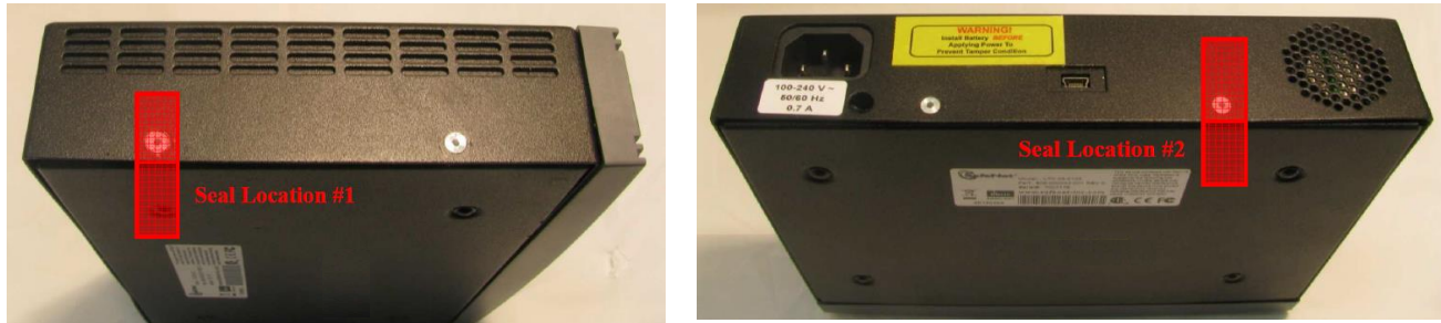
Figure 3-2. Tamper Evident Label Locations
