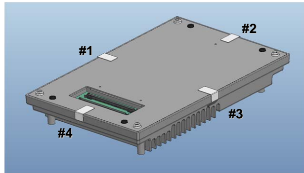
Figure 3 – Seal Location
