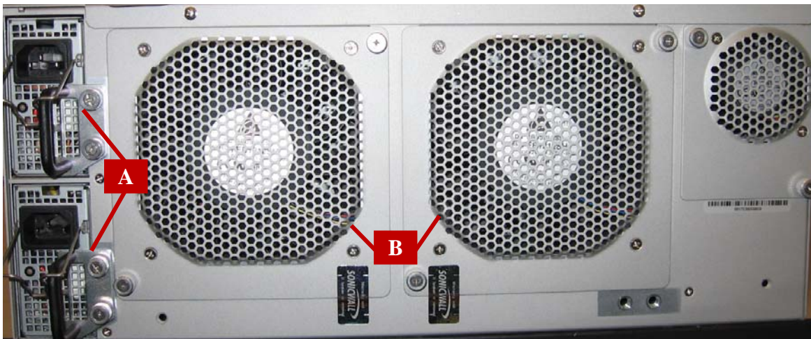
Figure 2 – NSA E10000 Back Panel
