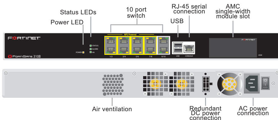
Figure 2: FortiGate-310B and 311B Front and Rear Panels
