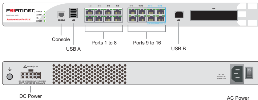
Figure 1: FortiGate-200B Front and Rear Panels
