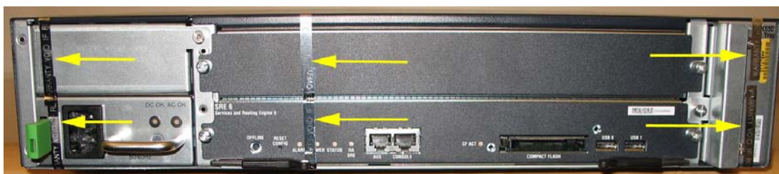
Figure 12. SRX650 Tamper Evident Seal Location (Rear)
